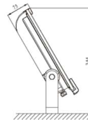
Seat-mounting
