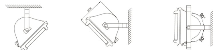
Ceiling mounting
